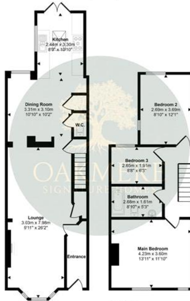
First Floor Approx 42 sq m / 449 sq ft
